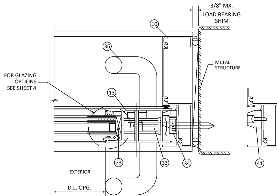
G 6 HORIZONTAL SECTION JAMB - THROUGH FRAME OPERABLE PANEL
