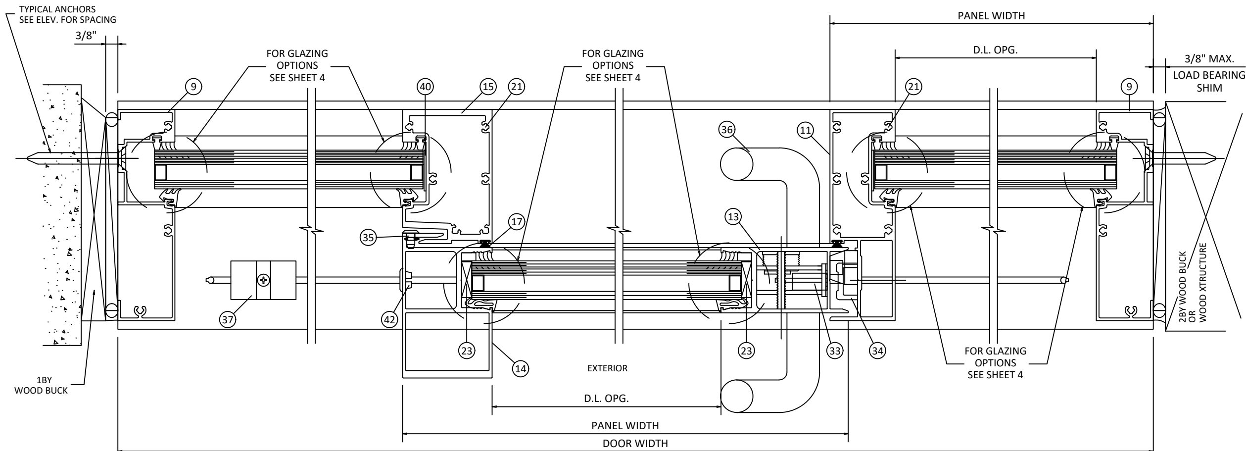
C 6 HORIZONTAL SECTION JAMB - THROUGH FRAME FIXED PANEL
